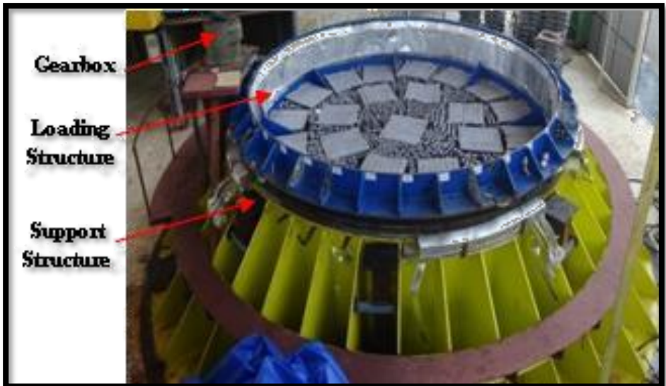
Facility for functional testing and qualification of large diameter bearing at IGCAR
