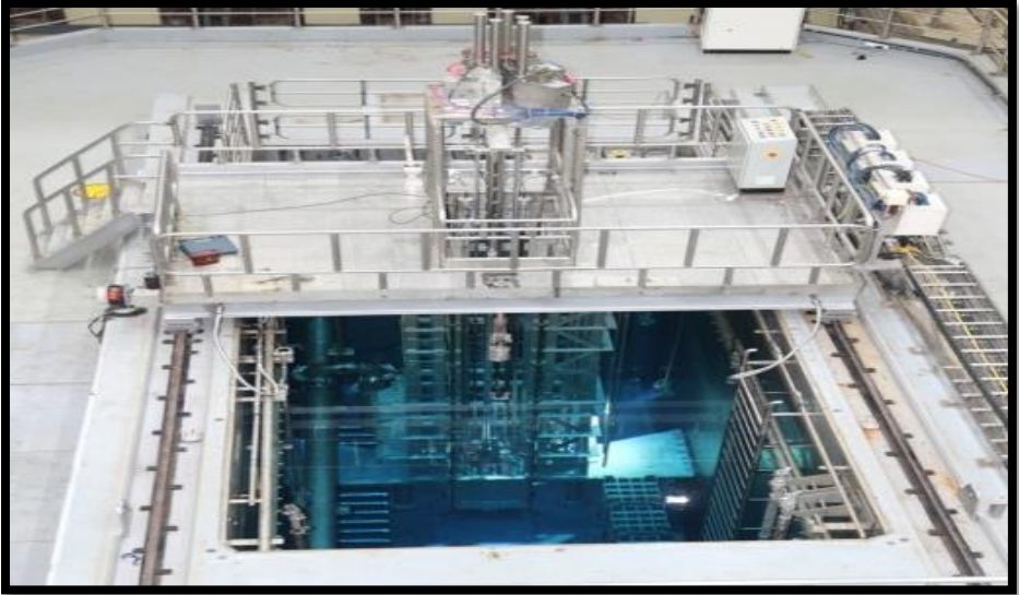
APSARA-U, Research Reactor at BARC
