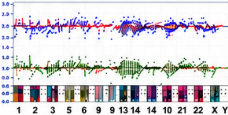
KaryoView
